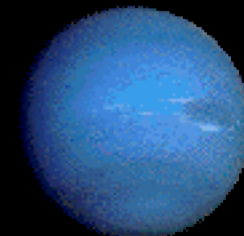
Neptune
